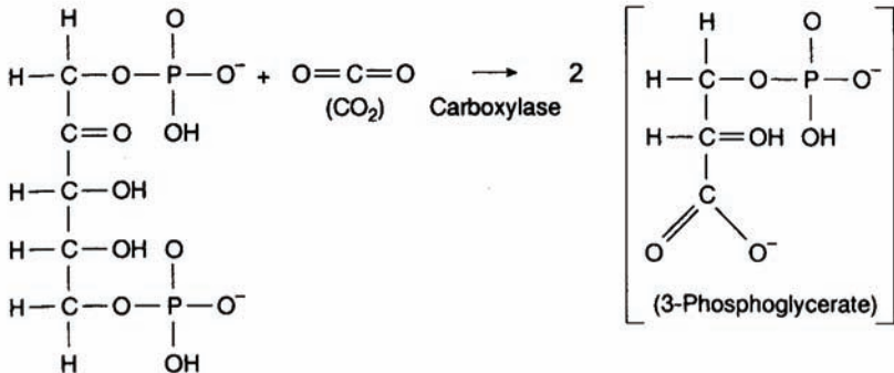
(Ribulose-1,5-bisphosphate)
