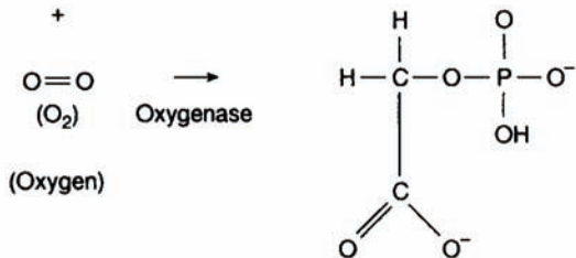
(2-Phosphoglycolate)
